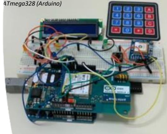
SSM/3G enabled, GPS device based on ATmega328 (Arduino)
